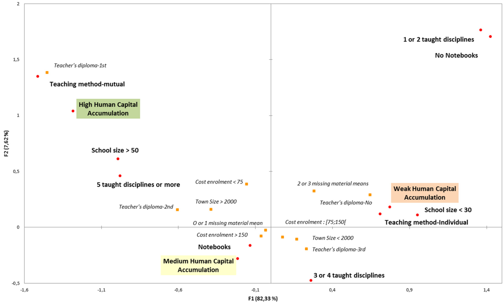
Graph 2. Multiple Factorial Analysis (axis F1 and F2 : 89,95 % of adjusted inertia)
